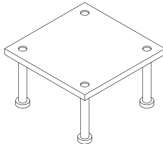
10" x 10" EMBED PLATE
